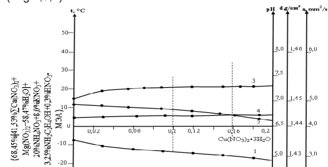
Fig. 2. Dependence of changes in crystallization temperature (1), pH (2), density (3) and viscosity (4) of solutions on the composition in the system {68.45%[ 41.53% \Sigma Ca(NO 3 ) 2 + Mg(NO 3 ) 2 + 58.47% H 2 O] + 20% NH 4 NO 3 + 8.0% KNO 3 + 3.25% NH 2 C 2 H 4 OH + 0.3% HNO 3 • MEA} - Cu(NO 3 ) 2 • 3H 2 O
