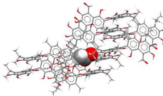
4-rasm. Gossipol va sirka kislotasi klatratining X-Ray tahlili
